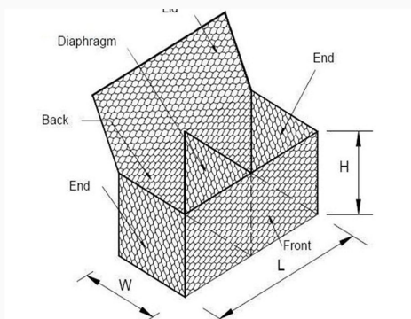
Specification Of Gabion Basket
